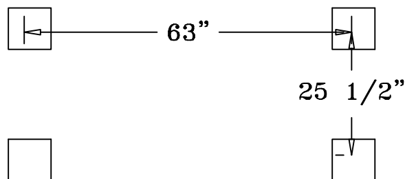
FOOTING DETAIL
