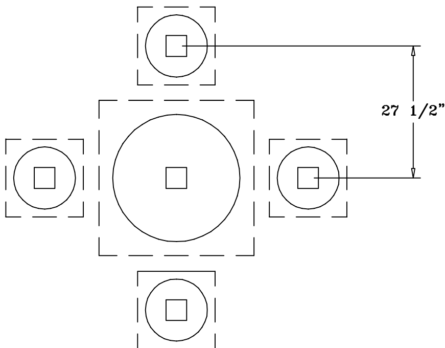
FOOTING DIAGRAM:
